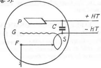
Fig. 3 -- Triode generator of very short waves, after the original drawing of Lakhovsky's patent.
