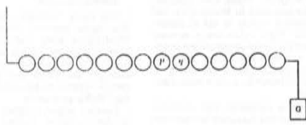
Fig. 90. Multi-gap lightning arrester.
