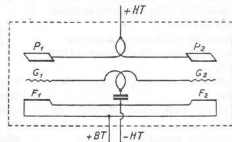
Fig. 5 -- According to the original drawing of the author's patent. Multiple triode including inside the bulb the connections of a symmetrical short-wave transmitter, with filaments set up in parallel.
