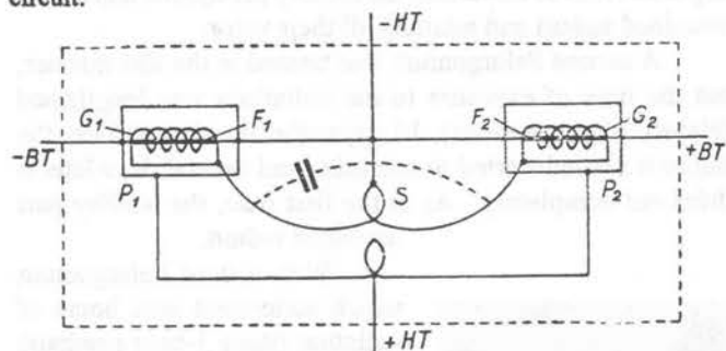
Fig. 6 -- Multiple triode symmetrically connected with filaments in series, according to the original drawing of the author's patent.
