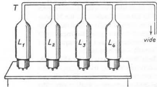
Fig. 4 -- Glass tube T helps maintain the same vacuum pressure inside the four triodes of a classic resonance receiver. Author's realization.
