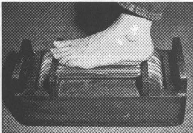
"Foot Fixer". This device uses a small Tesla coil to drive alternating tubes of argon and neon. Exact use and manufacturer unknown. Probably used to stimulate circulation.
